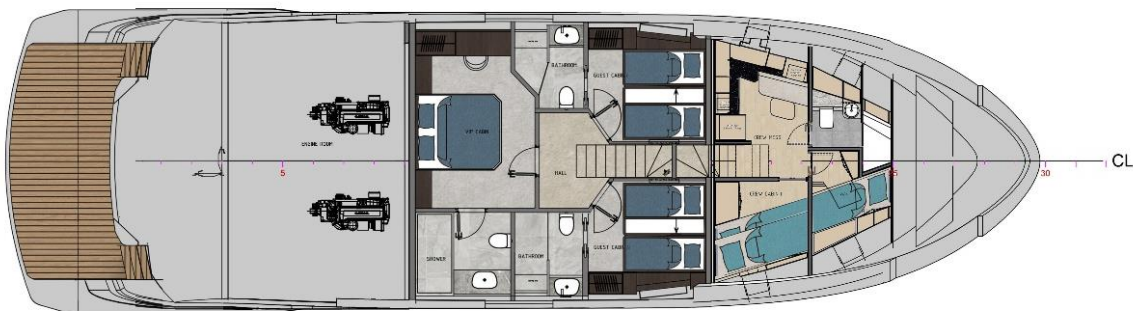
LOWER DECK PLAN
